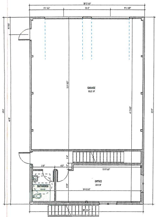
① GROUND FLOOR ARCHITECTURAL PLAN 1/4" = 1'-0"
