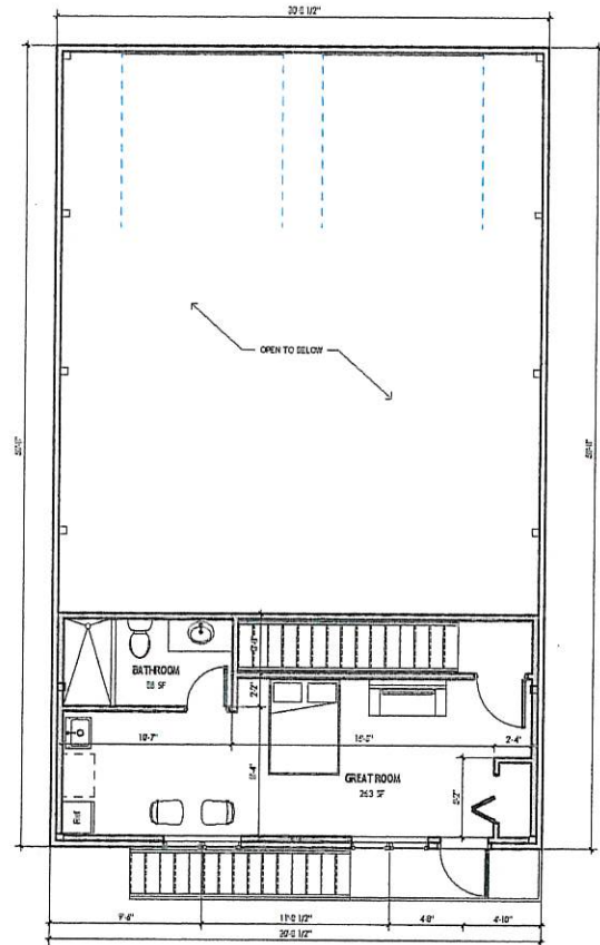
② SECOND FLOOR OPTION 1 1/4" = 1'-0"
