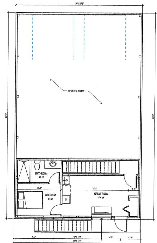
③ SECOND FLOOR OPTION 2 1/4" = 1'-0"
